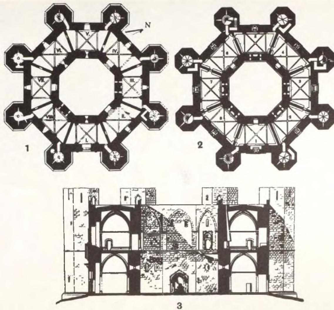
PLATE 30.—Plans and section of Castel del Monte (courtesy of Dr. Cresswell Shearer). 1. Ground-floor plan. 2. Upper-floor plan. 3. Section.
